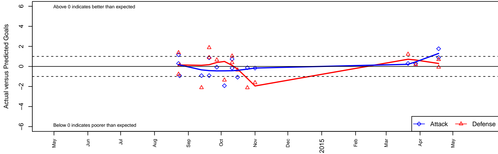
Spokane Spiders B02 Dots are actual minus expected GF (blue circles) and GA (red triangles). Blue line is smoothed change in attack strength. Red is smoothed change in defense strength.
